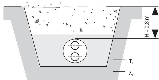
Abb. 25: pipe trench DUO-Rohr
