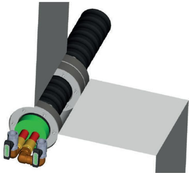
Abb. 48: Ring seal DW60 and NDW30 installed
