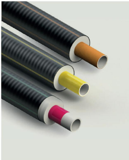
Abb. 1: up: FibreFlex PRO -pipe; middle: FibreFlex -pipe; under: HeatFlex -pipe
