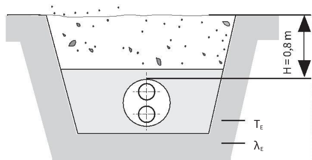
Abb. 23: Pipe trench DUO pipe
