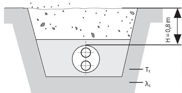
Abb. 21: Pipe trench DUO-pipe
