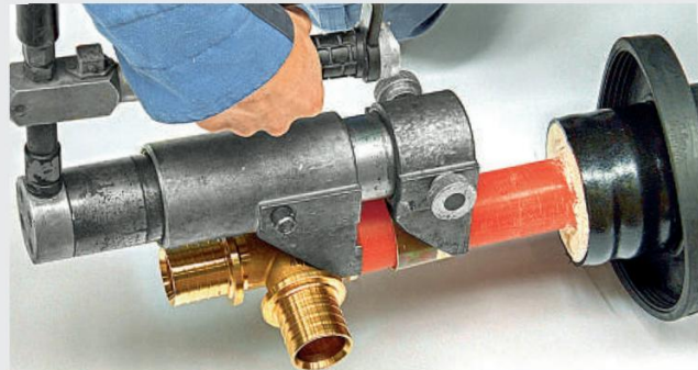
Pull the sliding sleeve over the body protector/ support. The connection is good if the medium pipe covers the last bar on the support body.
