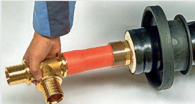
Insert the support body up to the last bar.
