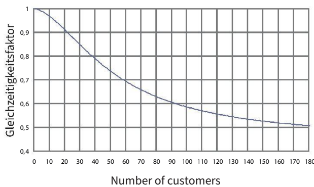
Diagram 1: Simultaneity of given building under the use of a transfer station
